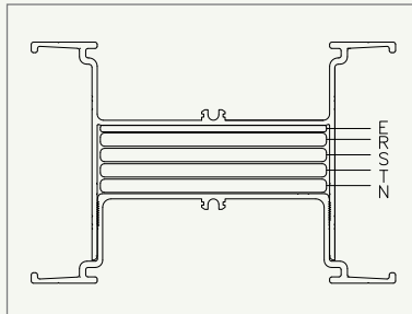
[4W+50%E, 100%E]
